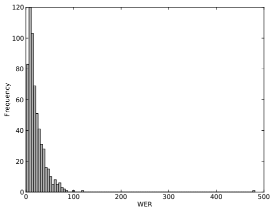
(a) ABBYY FineReader
