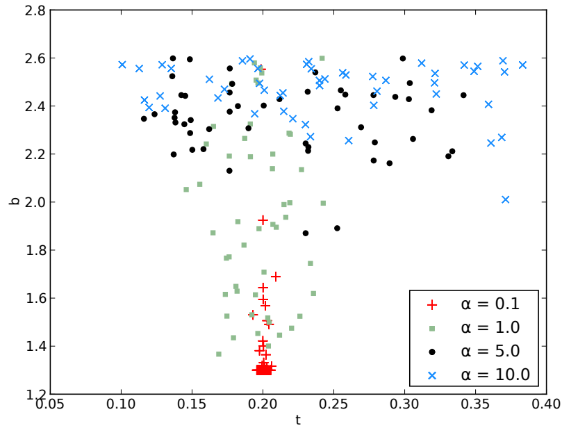
Figure 5.3: Samples of (b, t) parameter pairs at four different \alpha values. Fifty points were drawn for each \alpha value.
