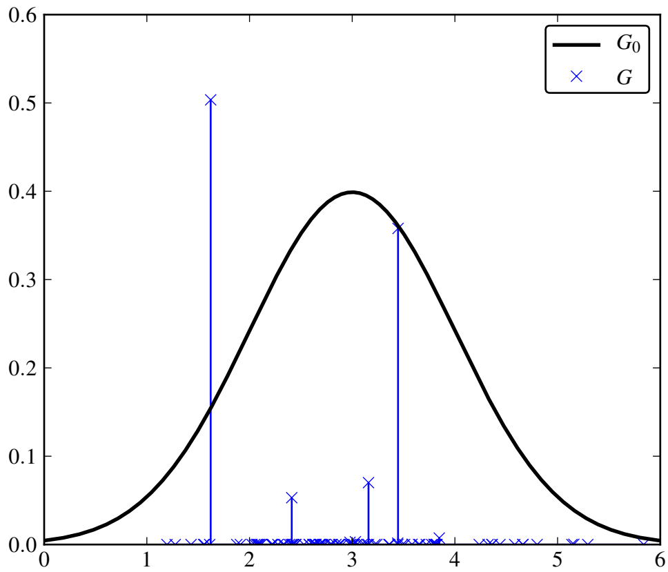
Figure 1.3: A finite approximation of a probability measure G drawn from a Dirichlet Process with G_0 = Normal(3, 1) and m = 1
