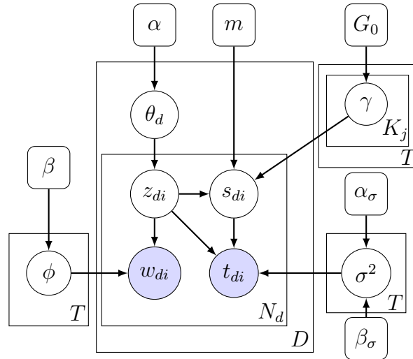
Figure 6.3: TONPT as used in sampling.
