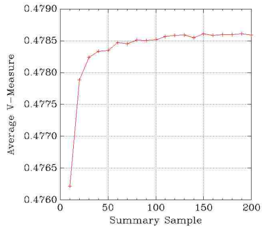
(b) Average V-Measures.
