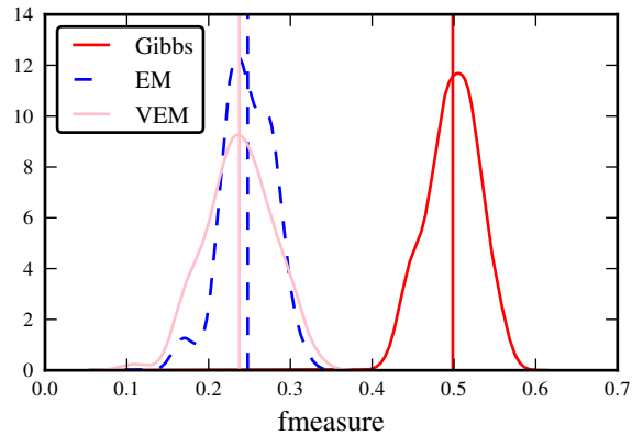
(a) F-measure
